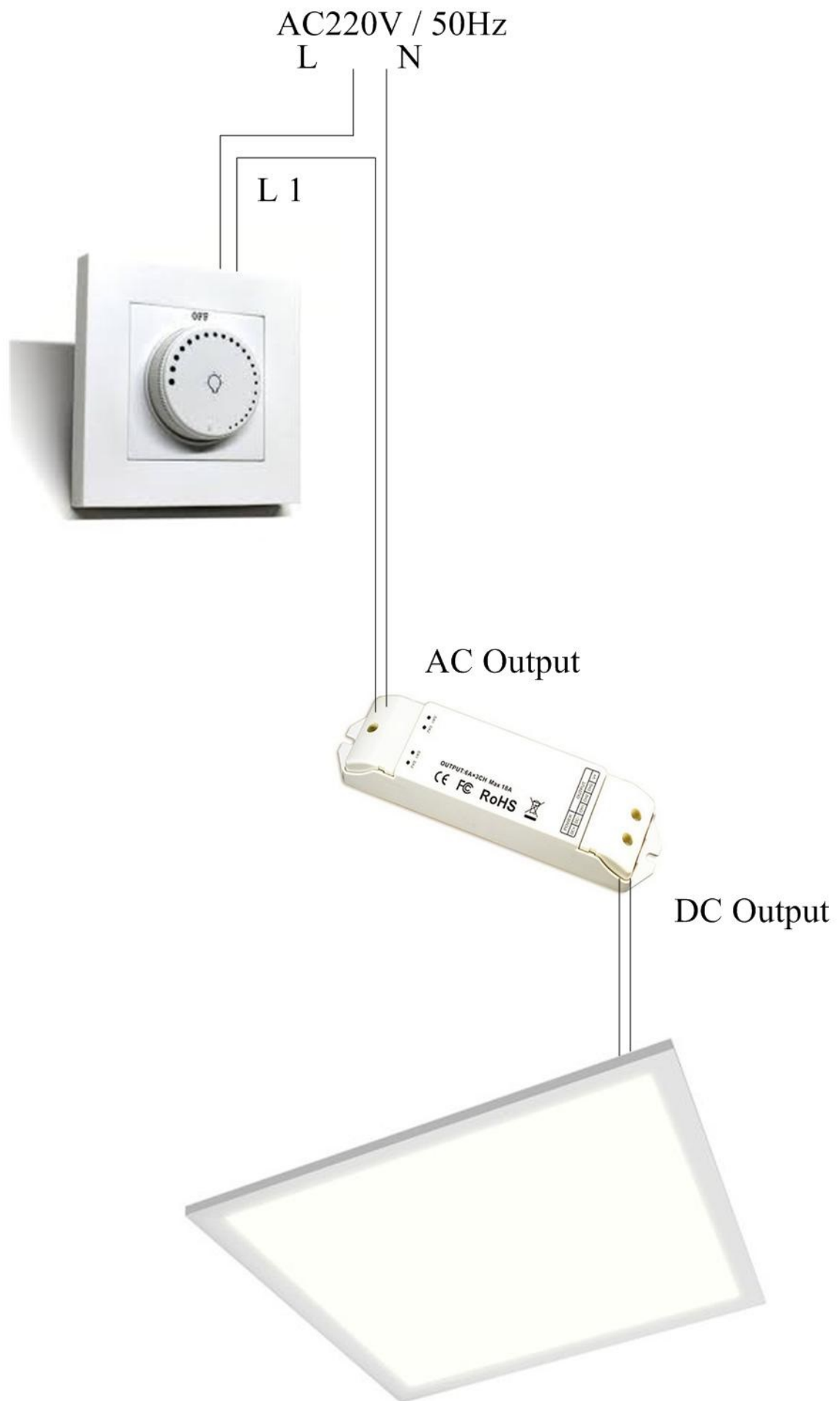
Phase control dimming for Panel light wiring diagram
