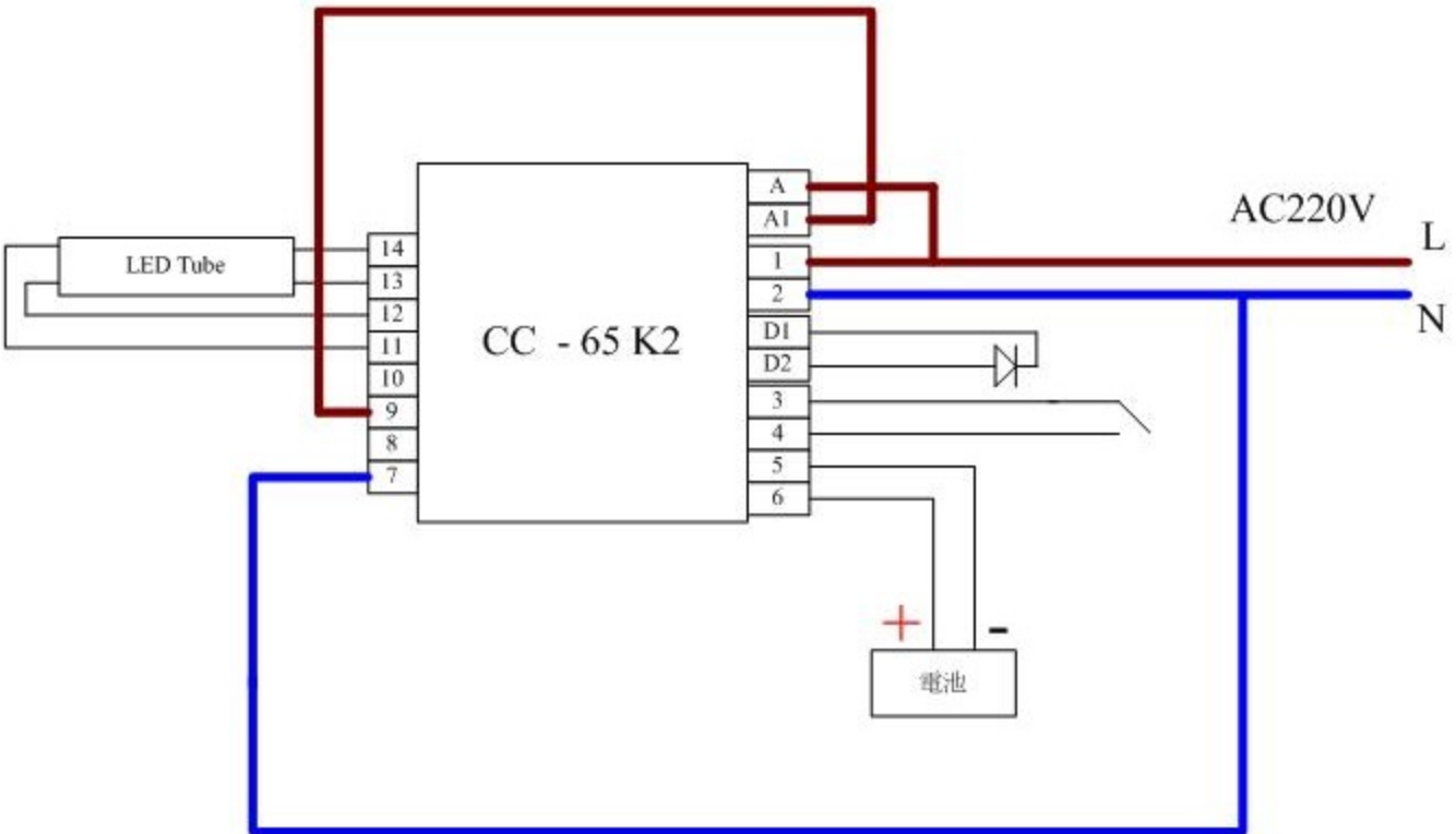
CC - 65 K2 wiring diagram for lighting LED tube - Double Side
