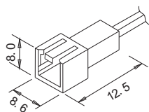
female socket
