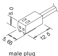
male plug
