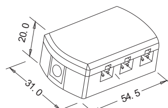
6-way distributor
