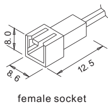
female socket
