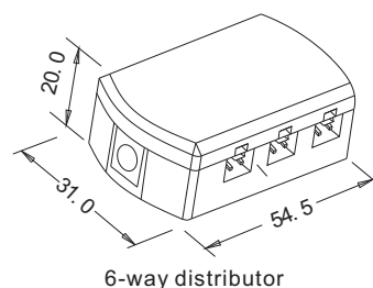
6-way distributor
